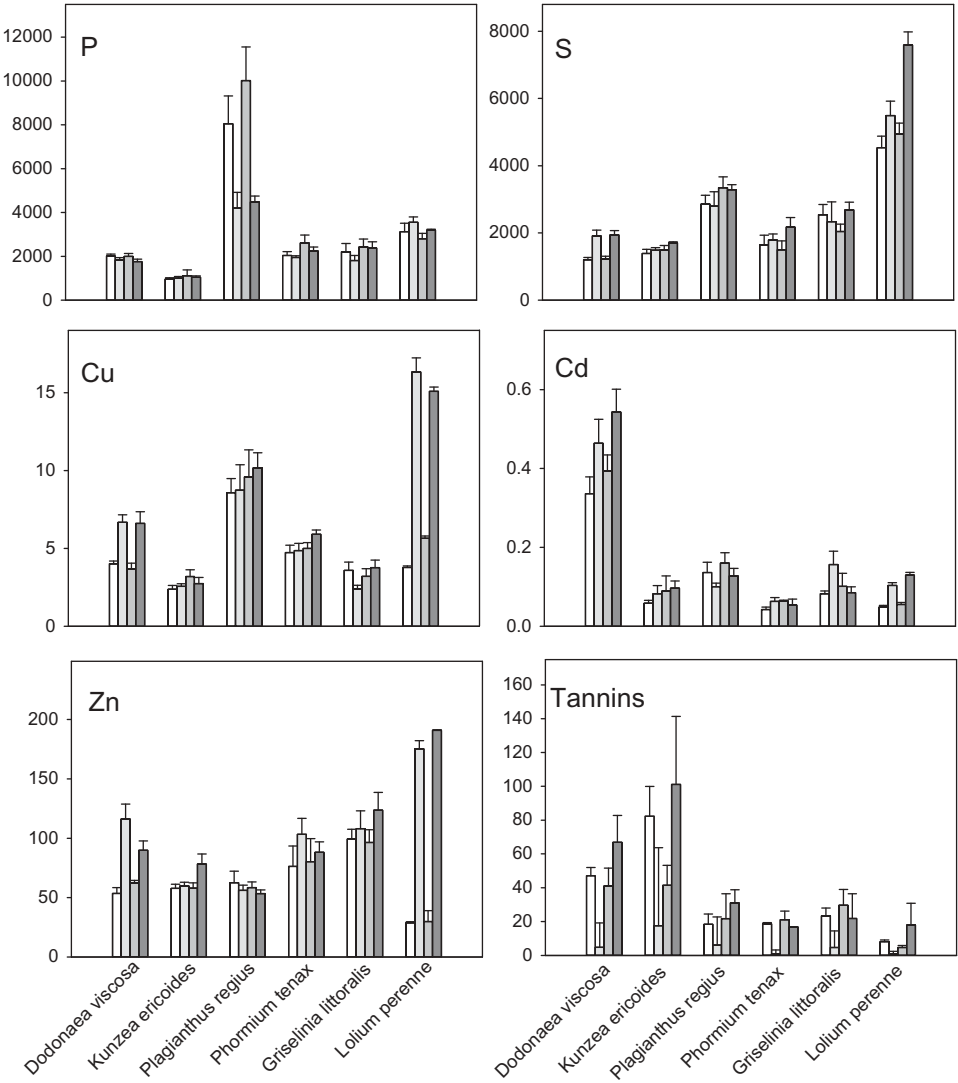
FIGURE 5 Elemental and tannin concentrations in plant foliage after growth in reference soil (open bars), soil with 10% biosolid amendment (lightest gray bar), soil with 20% biochar amendment (medium gray bars) and both amendments (dark gray bars), after 4 months growth in the pot experiment.
