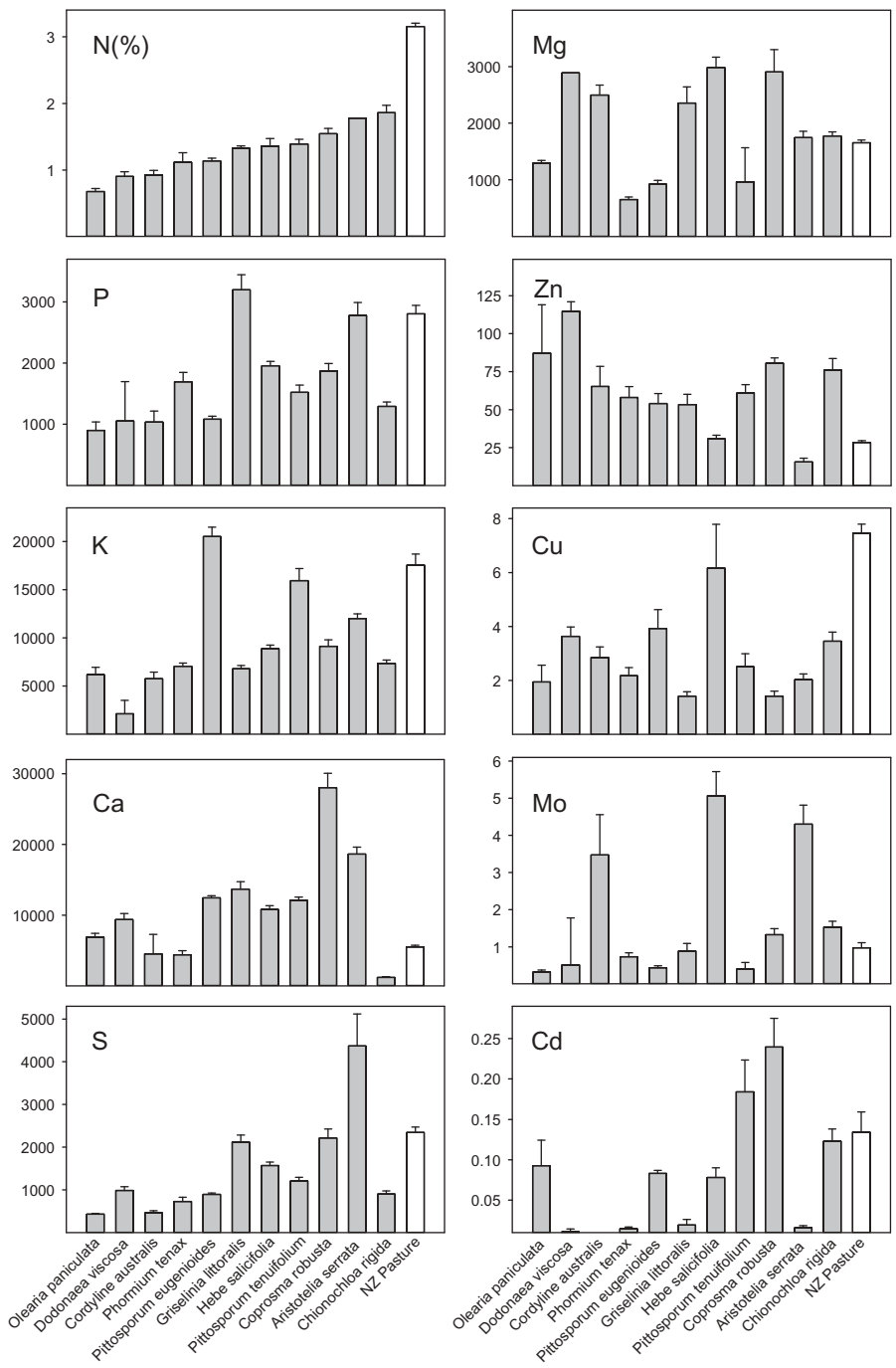
FIGURE 1 Concentrations of 10 elements in foliage sampled from nursery-grown native plants (aged <2 years), compared to published values for NZ pasture ryegrass. Values for N% in ryegrass are a mean of 7 urea and urine \pm DCD and control treatments ( n = 16 for each treatment) in field plots of the same farm from (Moir, Malcolm, et al. 2012). Values are \mu\text{g g}^{-1} (except N) \pm standard errors.
